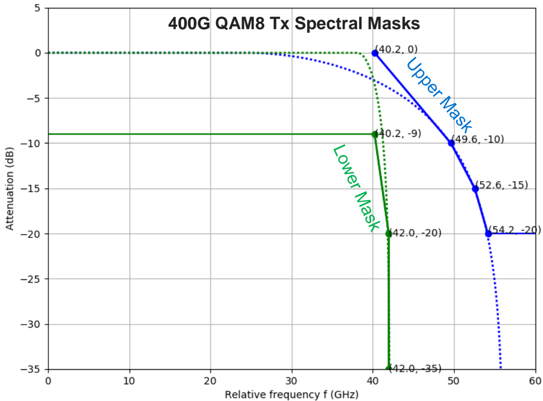
Figure 11-4x Transmit spectral masks (max and min)
