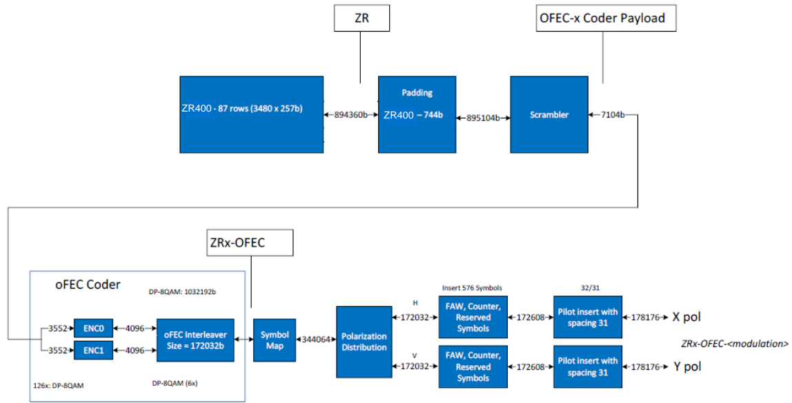
Figure 6-2a: Digital processes of ZR400 to ZR400-OFEC-8QAM adaptation.
