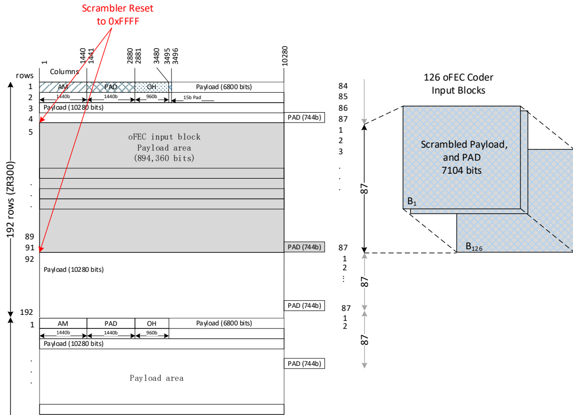
Figure 6-5: ZR300 adaptation to a ZR300-OFEC-8QAM line interface
