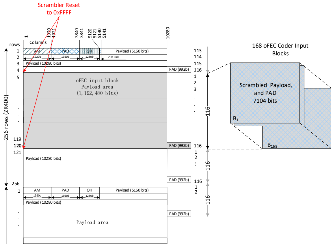
Figure 6-3: ZR400 adaptation to a ZR400-OFEC-16QAM line interface
