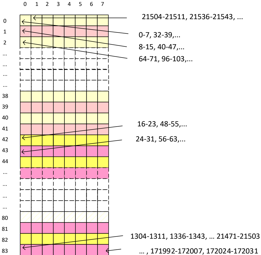
Figure 7-5: Inter-block interleaving
