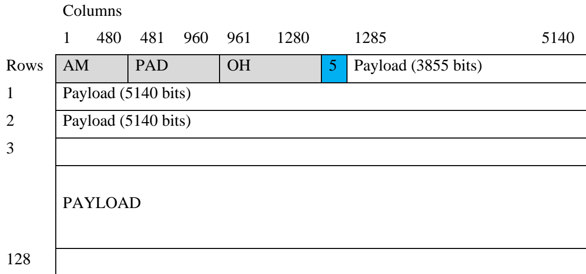
Figure 3-5 –ZR100 Frame
