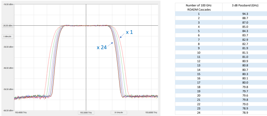
Figure 14-1: Illustrative 100GHz ROADM cascades (passband responses and 3dB bandwidth)
