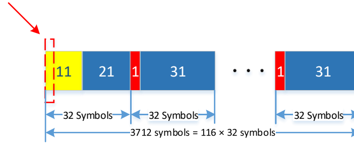
Figure 9-3: DSP sub-frames 1 to 47 of the DSP super-frame
