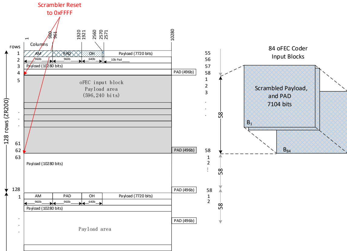
Figure 6-6: ZR200 adaptation to a ZR200-OFEC-QPSK line interface
