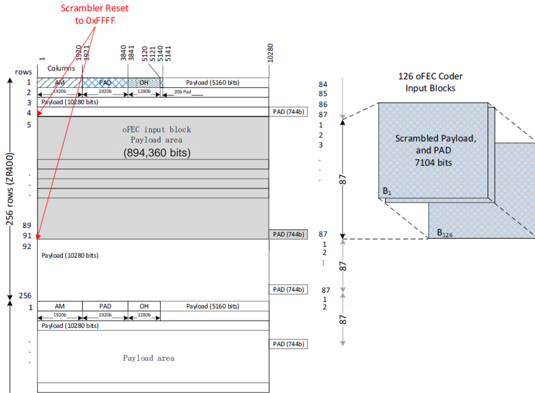
Figure 6-4a: ZR400 adaptation to a ZR400-OFEC-8QAM line interface
