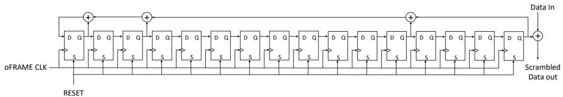
Figure 6-8: Frame synchronous scrambler
