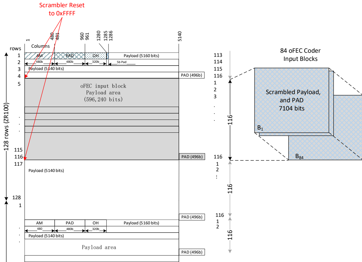
Figure 6-7: ZR100 adaptation to a ZR100-OFEC-QPSK line interface
